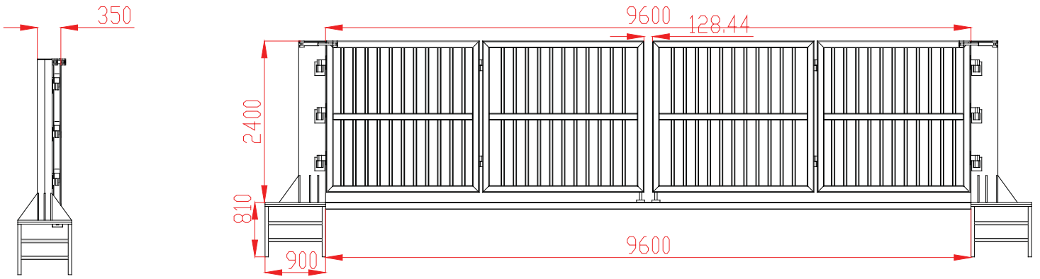
SIDE VIEW
