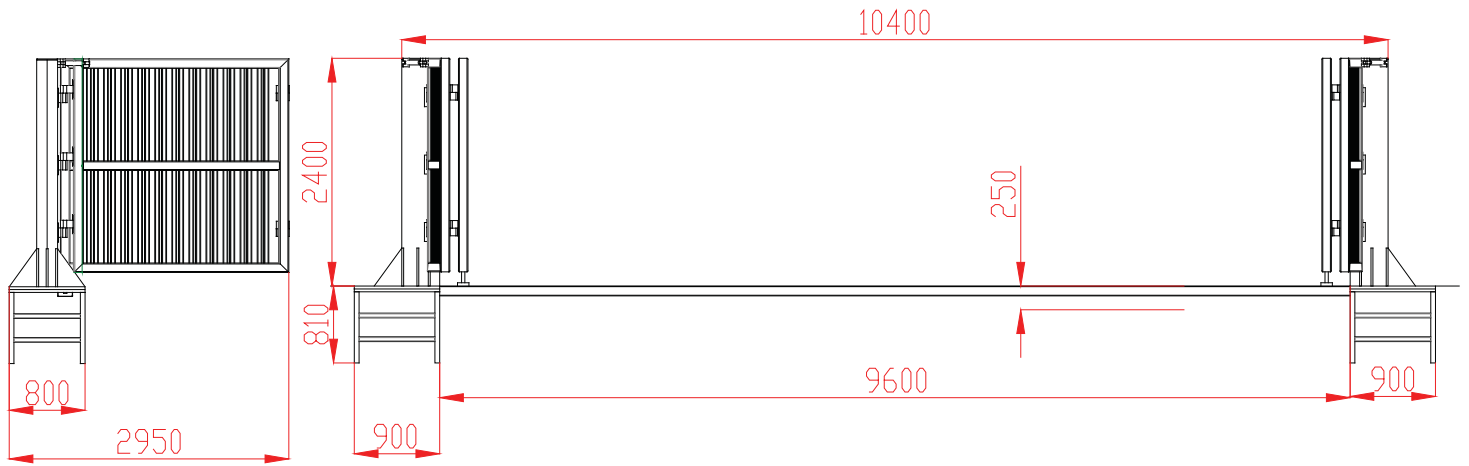
SIDE VIEW
